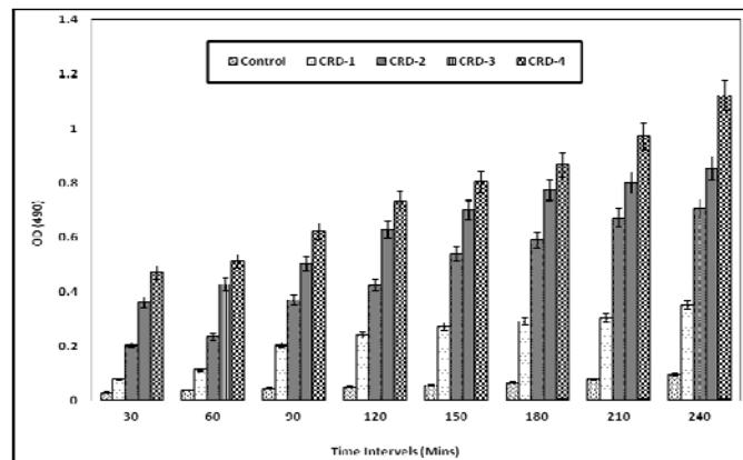
Fig. 3 Prophenol Oxidase (proPO) activity of haemocytes of F. indicus fed with C. rotundus extract enriched diets after WSSV challenge. The values significantly differed from each other (F= 91.09; P <= 0.0001)
