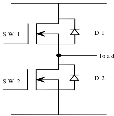
Fig. 4 One leg of a PWM inverter
