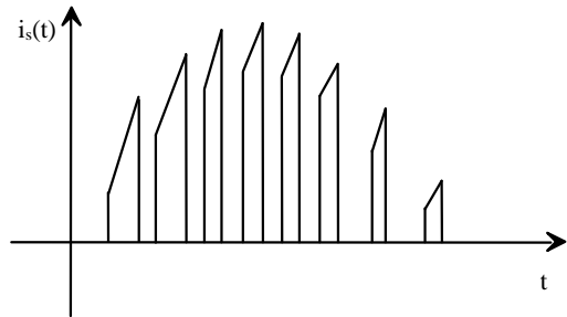
Fig. 6 The current waveforms of the top switch for one half cycle
