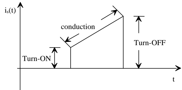
Fig. 7 The current waveforms of the top switch for one pulse
