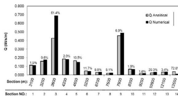
Fig. 4 Results of analytical and numerical groundwater seepage calculations into Amirkabir tunnel in 14 different sections. Values in the above of the columns show the relative difference between the seepage results of analytical and numerical methods
