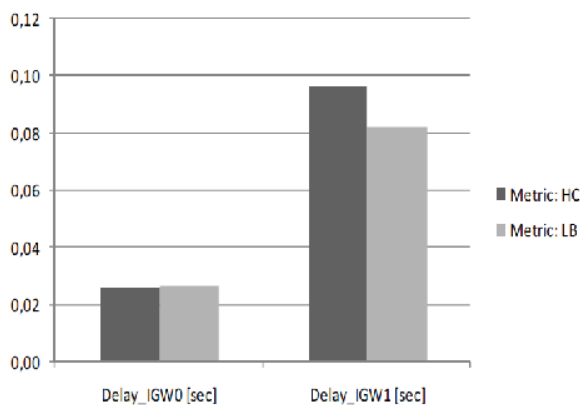
Fig. 7 Average Packet Transmission Delay [16]
