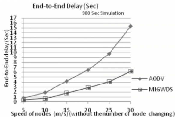
Fig. 8 End-to-End Delay of MIGWDS and AODV [11]
