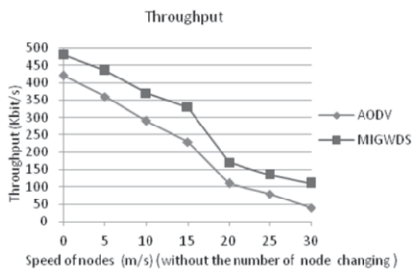
Fig. 9 Throughput of MIGWDS and AODV [11]
