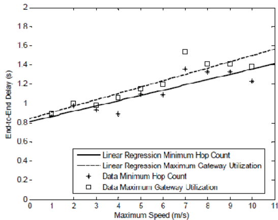
Fig. 5 End-to-End Delay versus Maximum Speed [3]
