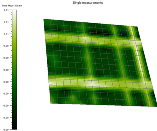
Fig. 11 X-direction 50MPa
