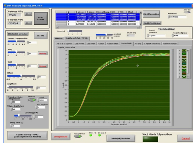
Fig. 5 Data storage & handling
