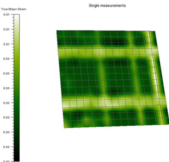
Fig. 12 Y-direction 50MPa
