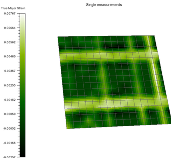
Fig. 13 X-Y direction 50MPa
