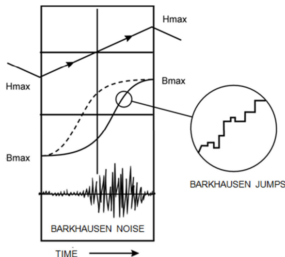
Fig. 1 Barkhausen effect
