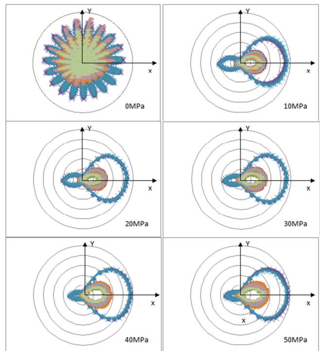
Fig. 15 Bi-axial stress state effect on BHN
