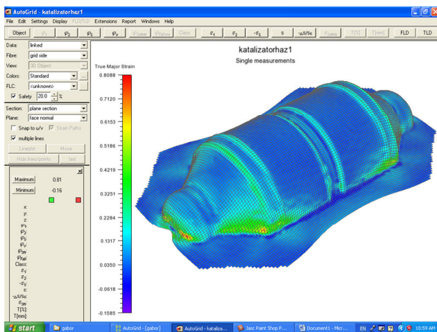
Fig. 8 Measuring of an automotive part by VIALUX system
