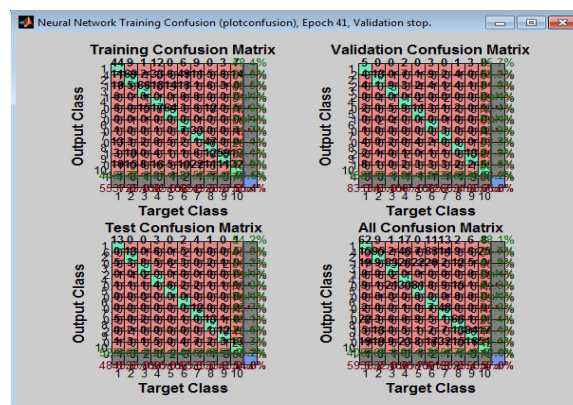
Fig. 8 Confusion Matrix
