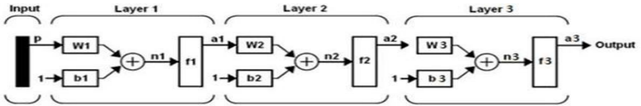
Fig. 4 Three-layer feed-forward neural network
