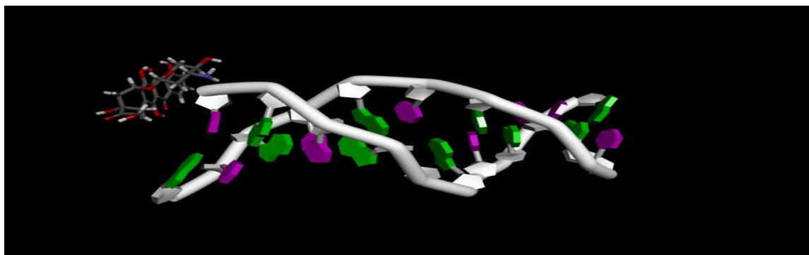
Fig. 5 Docked structure of DOX bound to Poly(dG-dC).Poly(dG-dC)
