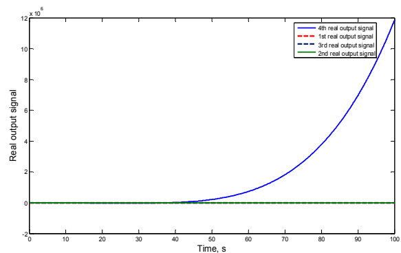
Fig. 4 Real output signal of 5MW wind turbine
