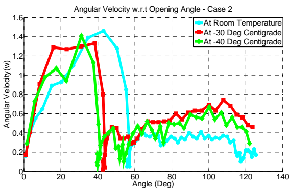
Fig. 10 Comparison of angular velocity with opening angle: case 2
