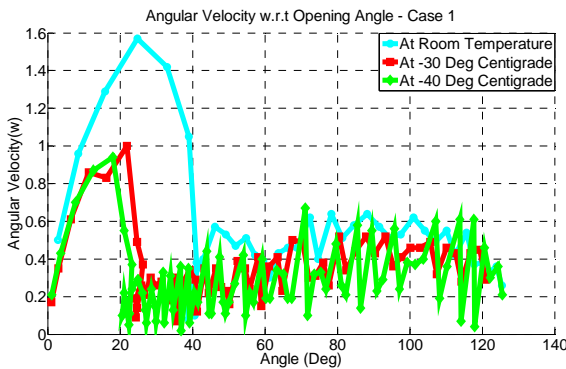
Fig. 8 Comparison of angular velocity with opening angle: case 1
