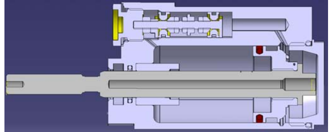
Fig. 2 Snubber internal parts
