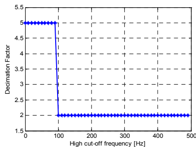
Fig. 2 Evolution of decimation factor with fault frequency
