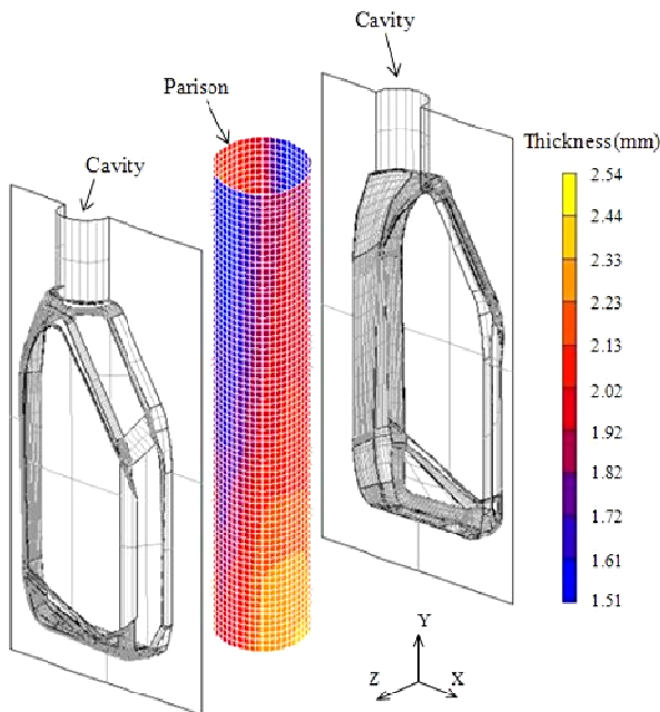
Fig. 3 The finite element model preparing for the blow molding simulation of a lubricant oil bottle
