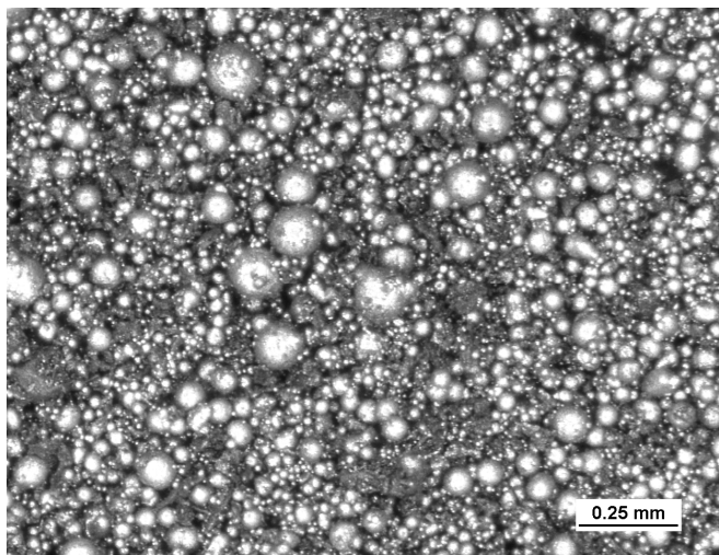
Fig. 1 Morphology of micro-nano powder mixture
