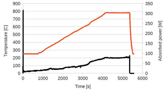
Fig. 2 Microwave sintering time-temperature and absorbed energy profile
