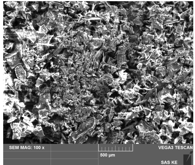
Fig. 3 SEM morphology of synthesized MnZn ferrite
