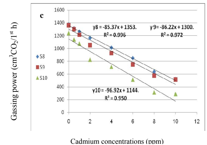
Fig. 5 (a) Effect of cadmium on gassing power of S. cerevisiae F-707, S. cerevisiae FA-91 and S. cerevisiae FF-725 strains; (b) Effect of cadmium on gassing power of S. cerevisiae F-235, S. cerevisiae F-25, S. cerevisiae FK-727, S. cerevisiae FK-727 and S. cerevisiae FC-620 strains; (c) Effect of cadmium on gassing power of S. cerevisiae FH-620, S. cerevisiae FAT-12 and S. cerevisiae F-514 strains
