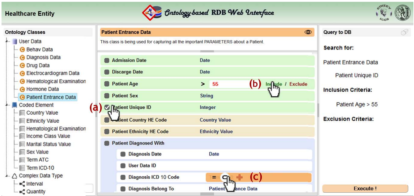
Fig. 2 A screenshot from the Ontology-based Web Interface for patient data as captured by a Healthcare Entity. (a) Selection of the parameters we should present for eligible entities, (b) Specifying an age criterion - in advance we have selected that it should be greater than the given value, (c) Pop-up window presented for introducing a diagnosis code restriction
