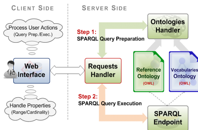
Fig. 3 The Web Tool (OntoQGenApp) Architecture
