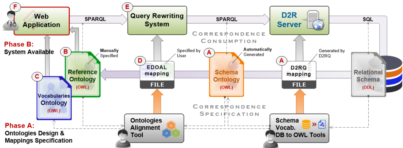
Fig. 1 The Steps we should follow for Linking the Web Application with a Relational Database
