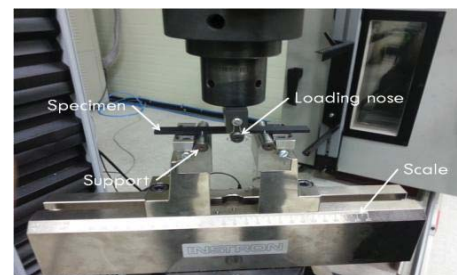
Fig. 3 Installed Specimen for Bending Test
