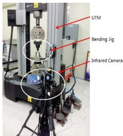
Fig. 4 Bending Test Experiment System
