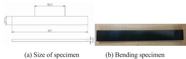
Fig. 2 CFRP Bending Test Specimen
