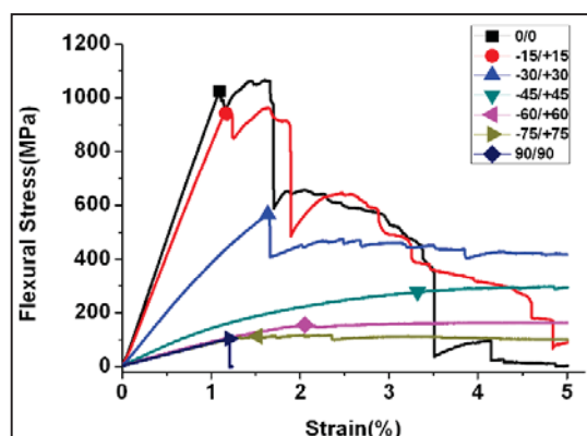
Fig. 5 Symmetry Bending Test result
