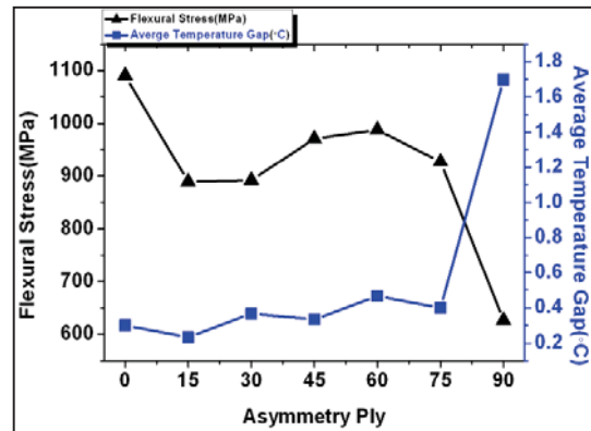
(b) Asymmetry Ply
