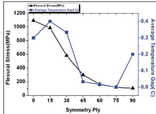
(a) Symmetry Ply
