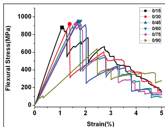
Fig. 6 Asymmetry Bending Test Result
