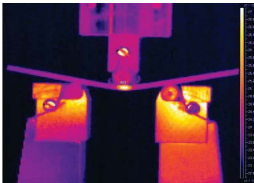
Fig. 8 Temperature Distribution of Bending Test
