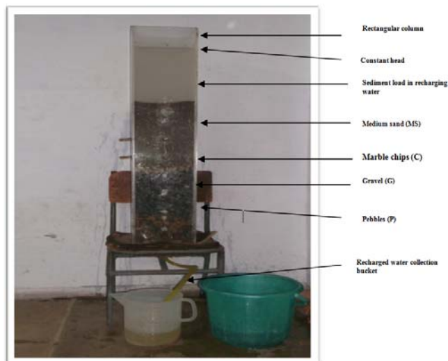
Fig. 1 Experimental column used in the laboratory study
