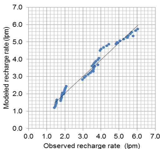
Fig. 2 Observed and modeled recharge rate using MLR
