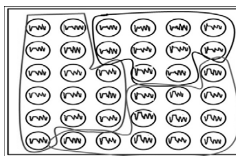
Fig. 3 SOFM map. The map is a 6 by 6 grid of nodes. Each spike is represented by a vector of EXPAR model coefficients. The SOFM decreases the dimensionality of dataset by finding the most probable patterns as the node weights. The similar patterns are assigned to neighbor nodes which are indicated by closed border
