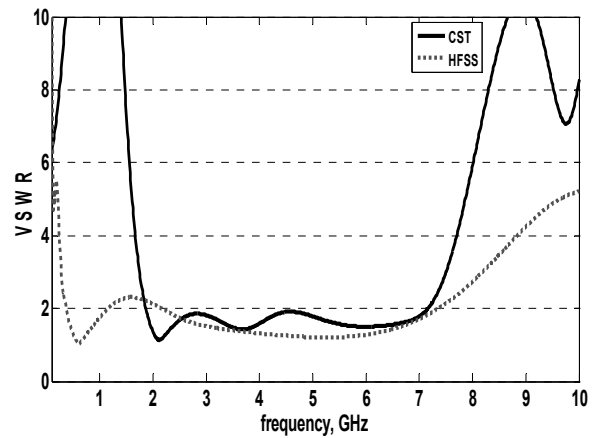
Fig. 6 VSWR of the proposed antenna with CST&HFSS
