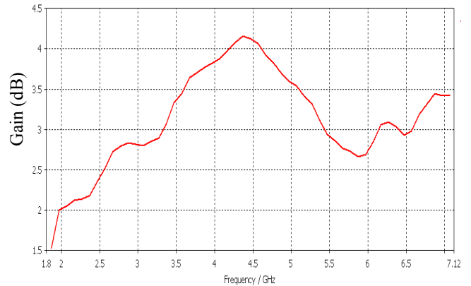
Fig. 7 The proposed antenna gain versus frequency
