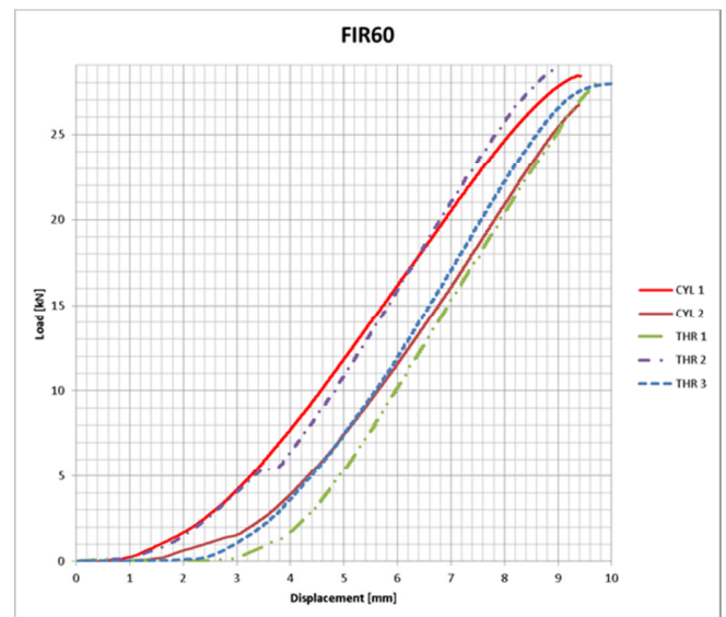
Fig. 10 Load-Displacement relationship in Douglas Fir samples
