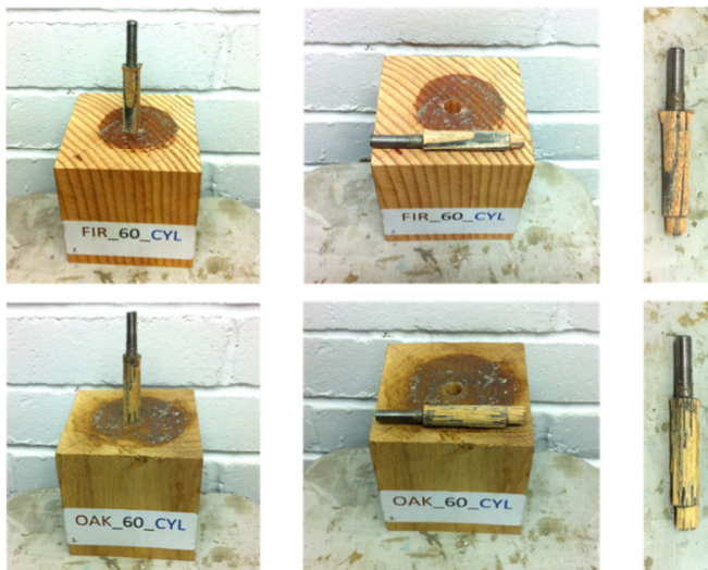
Fig. 12 Failure mode in Oak (bottom) and Douglas Fir (above) samples with smooth and cylindrical borehole after being tested by a pull-out test
