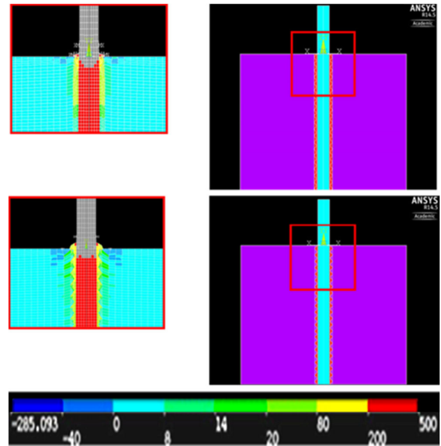
Fig. 15 Finite element models of glued in rod joint with threaded borehole (bottom) and cylindrical borehole (above). The scale range is expressed in MPa
