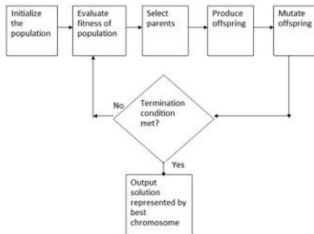
Fig. 4 Genetic Algorithm flowchart [5]
