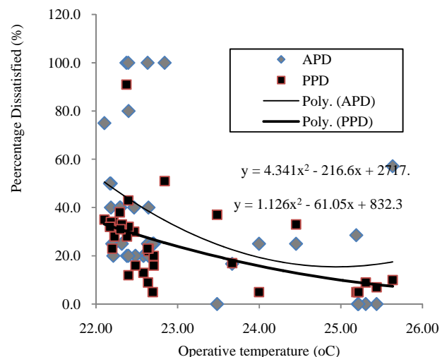
Fig. 4 Graph of percentage dissatisfied versus operative temperature
