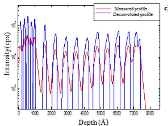
Fig. 2 (c) Evolution of the deconvoluted profile depending on the number of iterations n ( n=10000 )
