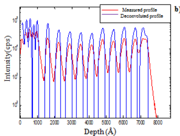
Fig. 2 (b) Evolution of the deconvoluted profile depending on the number of iterations n ( n=1000 )
