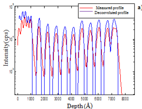
Fig. 2 (a) Evolution of the deconvoluted profile depending on the number of iterations n ( n=200 )
