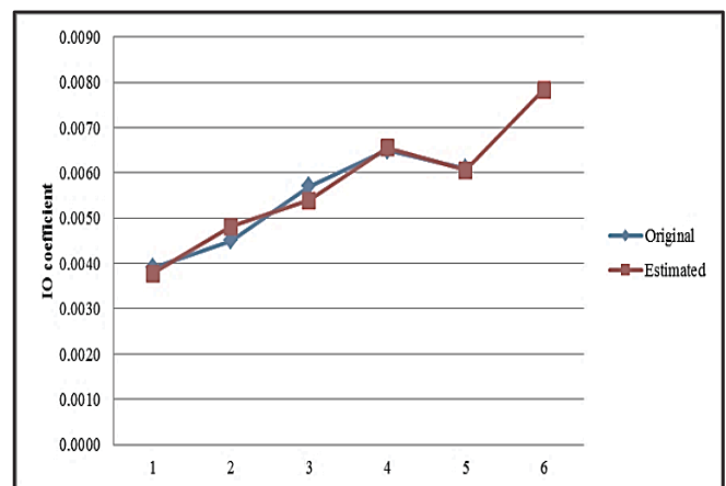
Fig. 4 The changes in a_{72,59} from 1985-2015
