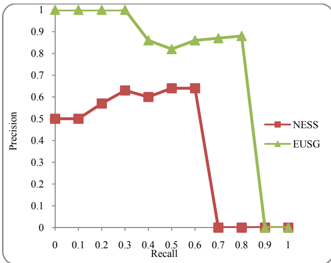
Fig. 3 Recall-Precision Graph of Update Summary at 20% CR
