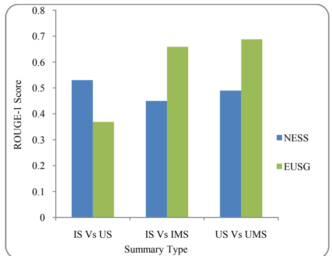
Fig. 4 ROUGE-1 Score Performance Measure
