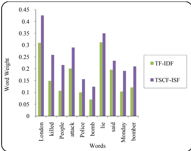
Fig. 2 Word Weight Measure Analysis
