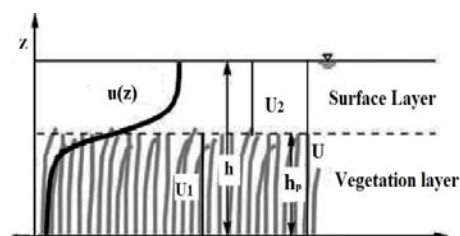
Fig. 1 Velocity profile within and above vegetation
