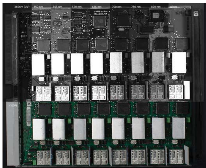
Fig. 11. Panel 3 - VIS compared to all single spectra
