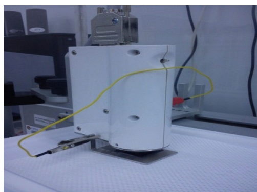
Fig. 4 KSV Surface Potential Sensor (SPOT)
