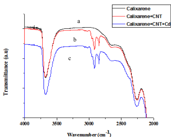
Fig. 5 FTIR spectra of (a) calix[8]arene, (b) MWCNTs-calix[8]arene nanocomposite and (c) MWCNTs-calix[8]arene with Cd 2+
