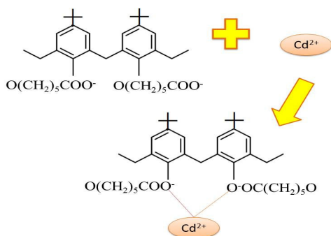
Fig. 3 The mechanism of calix[8] detection \text{Cd}^{2+} ions
