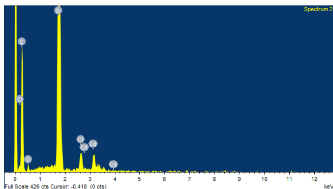
Fig. 9 EDX analysis of MWCNTs-calix[8]arene with \text{Cd}^{2+}
