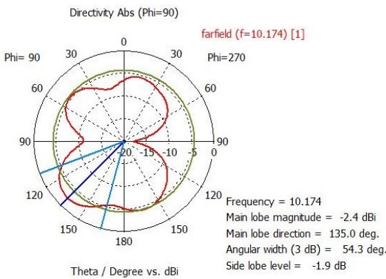
Fig. 8 The diversity radiation pattern E-plane of frequency 10.174 GHz simulated by CST Microwave.
