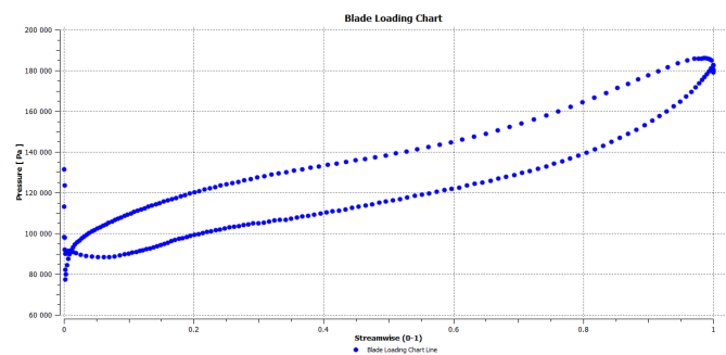
Fig. 3 The pressure diagram on the periphery blade to blade surface (ANSYS CFX)
