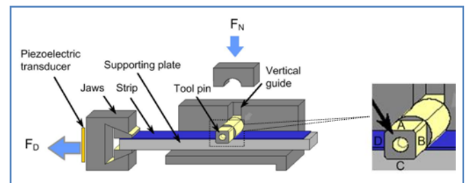
Fig. 3 The principles of the Strip Reduction Test experimental device
