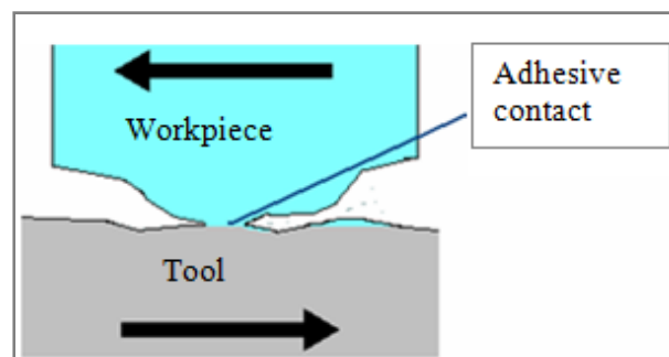
Fig. 1 Schematic illustration of adhesive wear
