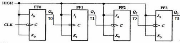
Fig. 1 4-bit binary counter using J-K flip flops
