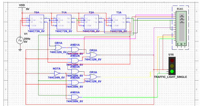
Fig. 2 4-bit binary counter using J-K flip flops
