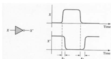
Fig. 5 The effect on propagation delay [8]
