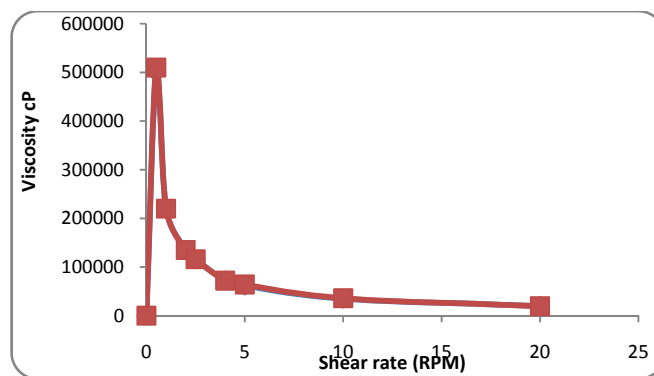
Fig. 8 Rheological behavior of SLNs hydrogel (n=3±SD)
