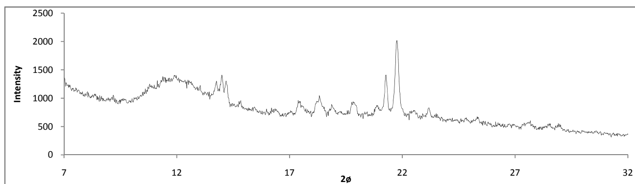
Fig. 9 Diffraction pattern of RISP
