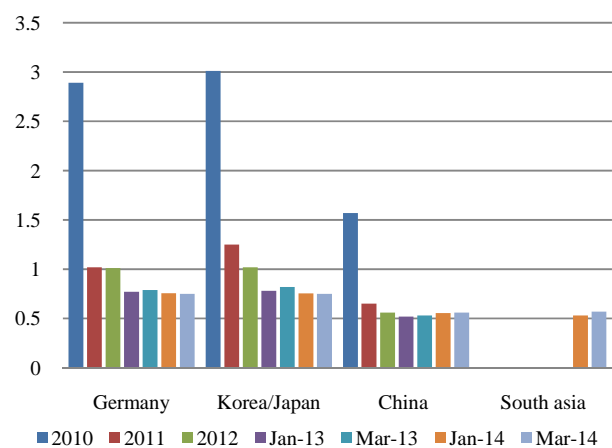
Fig. 7 Photo-voltaic cell experience pricing [4]
