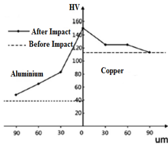
Fig. 13 Micro hardness in welding zone of Al/Cu
