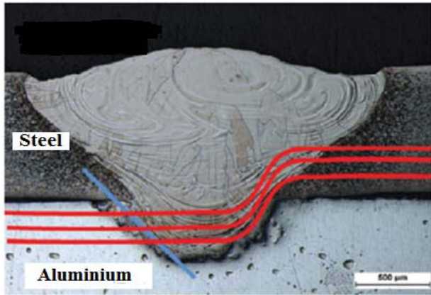
— Intermetallic phase boundary
