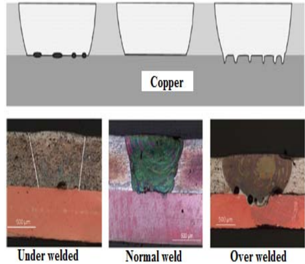
Fig. 14 Intermetallic seam structures
