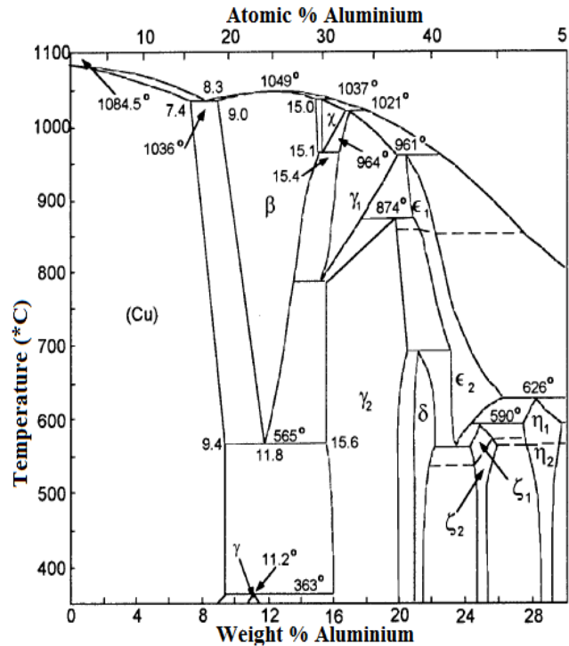
Fig. 3 Binary - Copper Aluminium phase diagram
