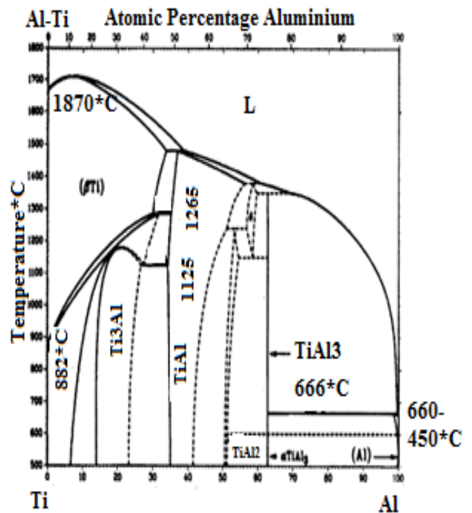
Fig. 1 Binary Ti–Al equilibrium phase diagram
