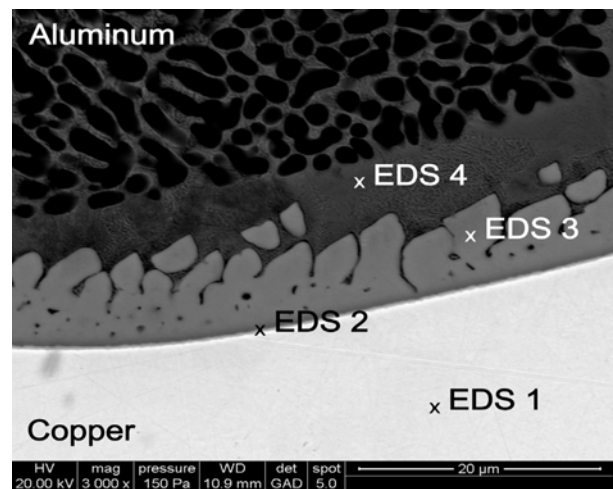
Fig. 12 IMC seam formation after laser beam braze welding
