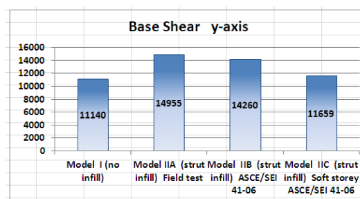
Fig. 15 (b) Base shear Y-Y
