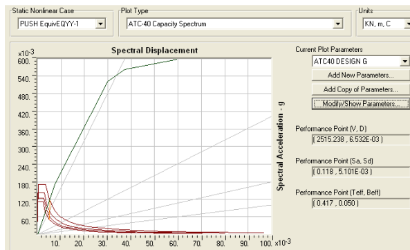
Fig. 17 (c) Model IIB (strut infill- ASCE/SEI 41), R=3.92
