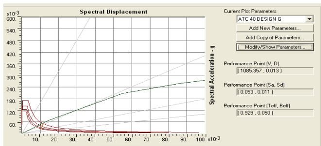
Fig. 16 (a) Model I (no infill), R=2.04
