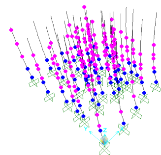
Fig. 13 (c) Model IIB (strut infill- ASCE/SEI 41)
