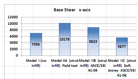
Fig. 15 (a) Base shear X-X
