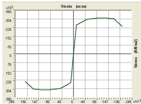
Fig. 11 (b) Stress-strain curve for steel bars
