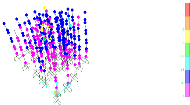
Fig. 14 (a) Model I (frame element +slab)
