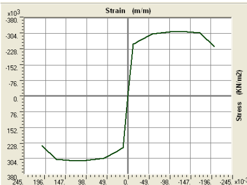
Fig. 6 (b) Stress-strain curve for steel bare
