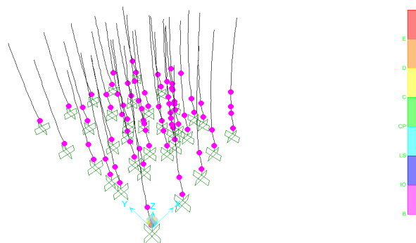
Fig. 14 (b) Model II (frame element +slab+ infill walls)
