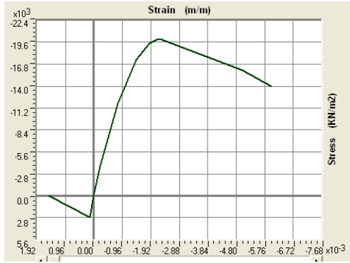
Fig. 6 (a) Stress-strain curve for concrete
