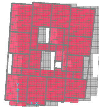
Fig. 10 (b) T_1=0.323 sec (Model II) infill wall
