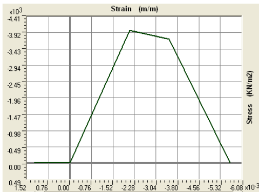
Fig. 6 (c) Stress-strain curve for clad brick
