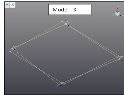
Fig. 9 Experimental mode shapes for the building
