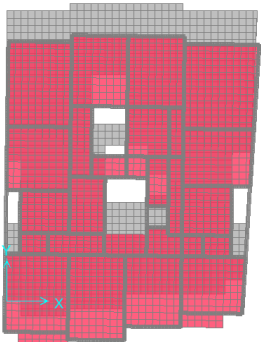
Fig. 12 (a) T_3=0.637 sec (Model I) no infill wall
