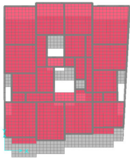
Fig. 11 (b) T_2=0.268 sec (Model II) infill wall
