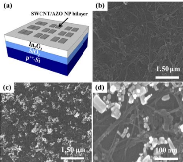
Fig. 1 (a) The SWCNT/AZO NP bilayer electrode TFT. SEM images of (b) SWCNT film and (c), (d) SWCNT/AZO NP bilayer film
