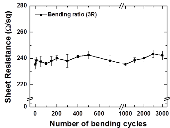
Fig. 3 Variations of the sheet resistance after the bending test of SWCNT/AZO NP bilayer film
