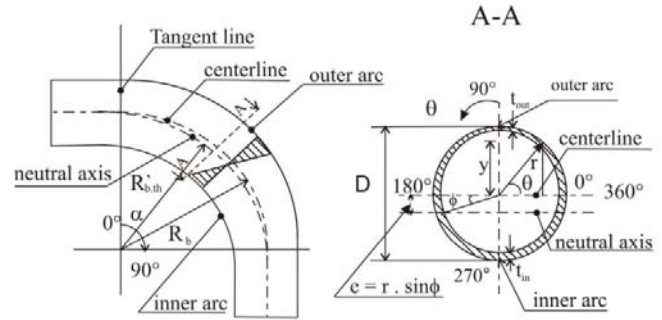
Fig. 3 Geometry of the tube and wall thickness distribution in rotary draw bending processes
