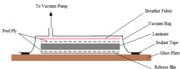
Fig. 1 Layup sequence for vacuum bagging
