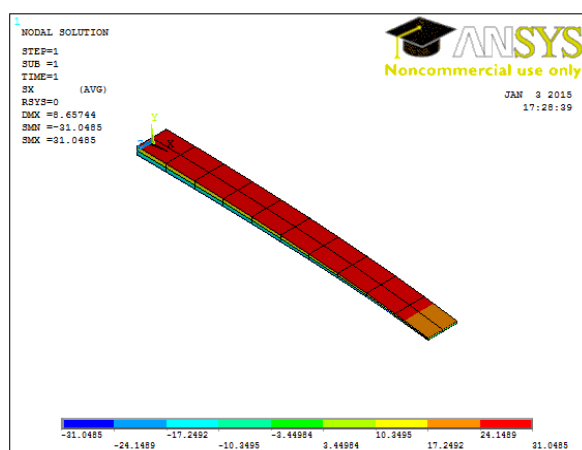
Fig. 6 Stress plot at Load P = 19.62 N
