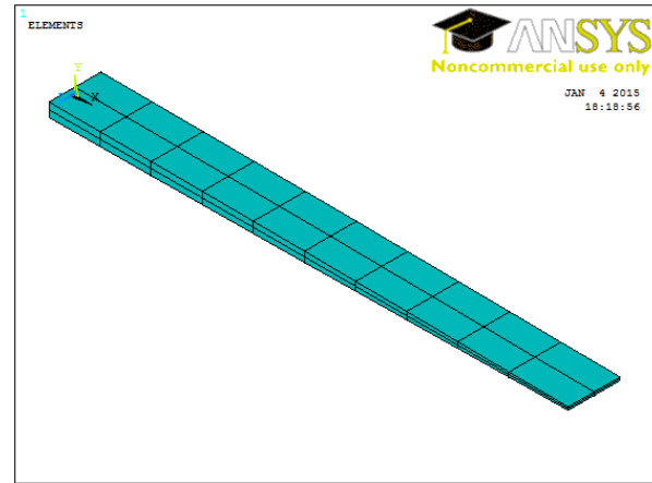
Fig. 5 Finite element model for constant stress beam
