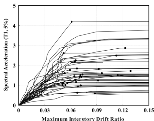
Fig. 2 Result of incremental dynamic analysis
