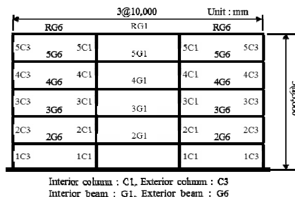
Fig. 1 Elevation and frame plan of prototype building
