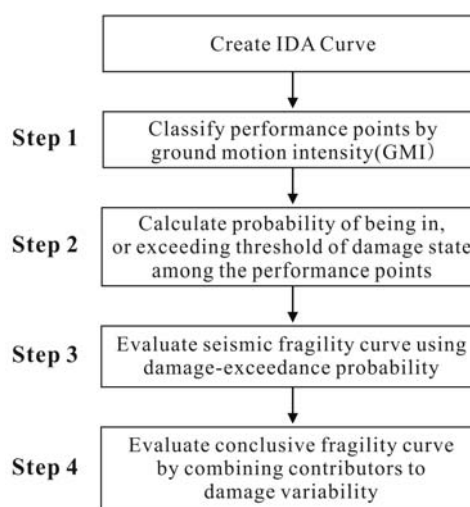
Fig. 3 Flowchart of procedure for calculating seismic fragility curve using IDA method
