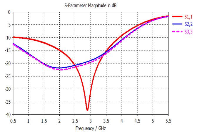
Fig. 11 Simulated return loss
