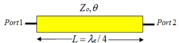
Fig. 3 The quarter wave-length transmission line
