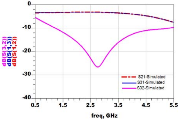
Fig. 8 Simulated transmission and isolation
