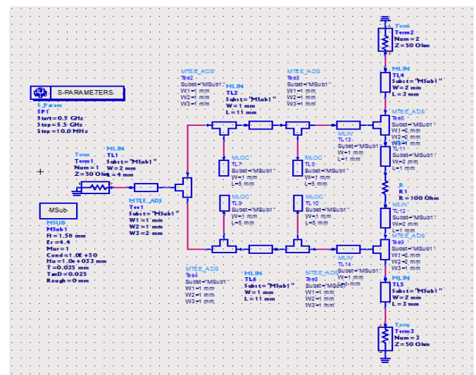
Fig. 6 The schematic of the power divider
