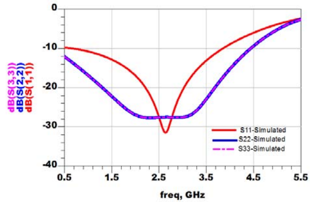
Fig. 7 Simulated return loss
