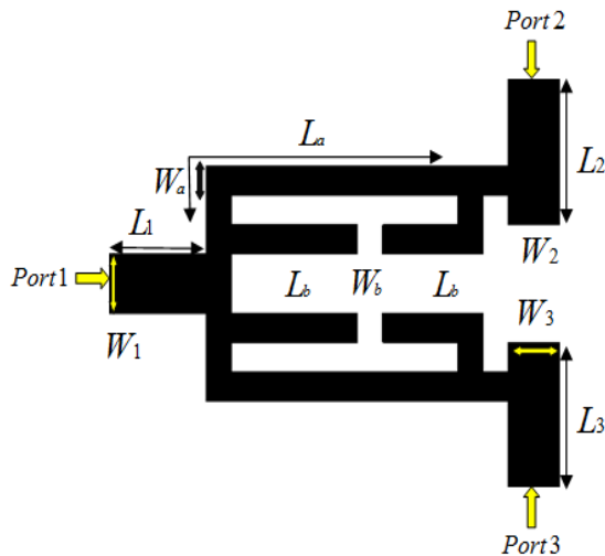
Fig. 5 Circuit the proposed power divider
