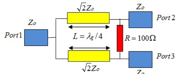
Fig. 1 The conventional Wilkinson power divider
