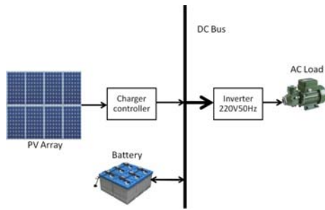
Fig. 1 PV Stand-Alone Energy System
