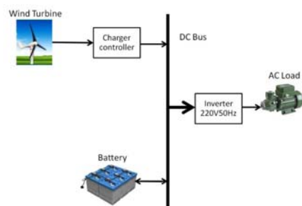
Fig. 2 The Wind Turbine Stand-Alone Energy System
