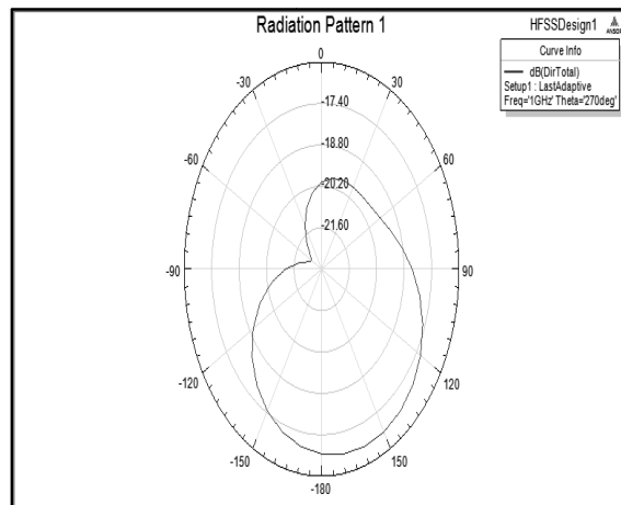
Fig. 4 Radiation pattern of proposed antenna
