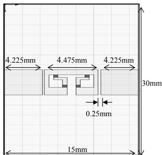
Fig. 2 Top section of Band pass filter
