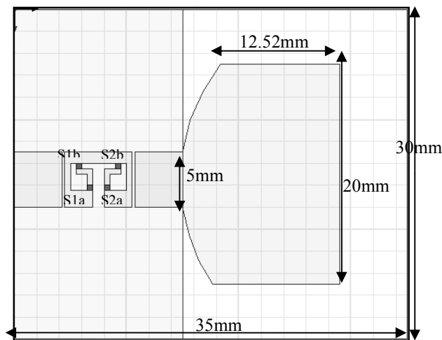
Fig. 3 Top section of single port overlay CR antenna
