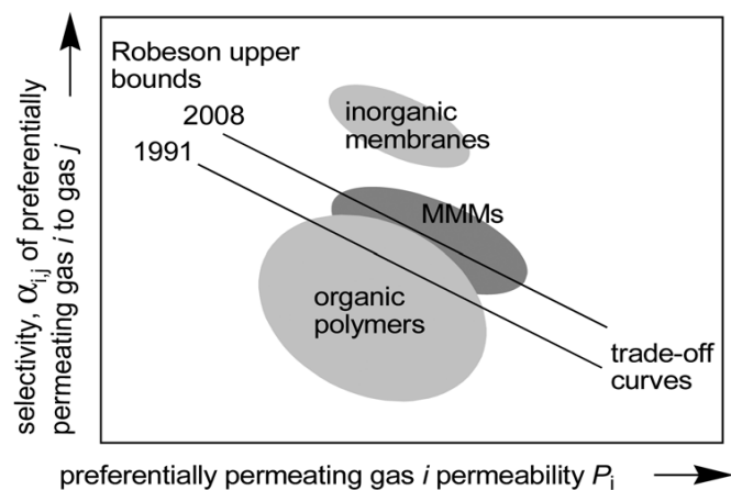
Fig. 1 Robesson graphs to compare different kinds of membranes for gas separation [9]
