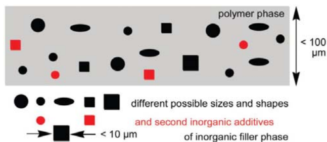
Fig. 2 Schematic of a mixed-matrix membrane [9]
