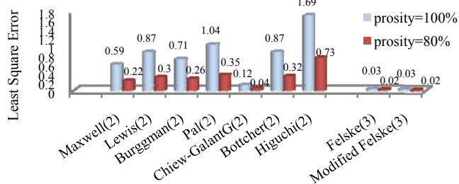
Fig. 5 Comparing error percentage of exist model with improved model with J coefficient for CO 2 separation of CO 2 /CH 4 in Matrimid/CMS
