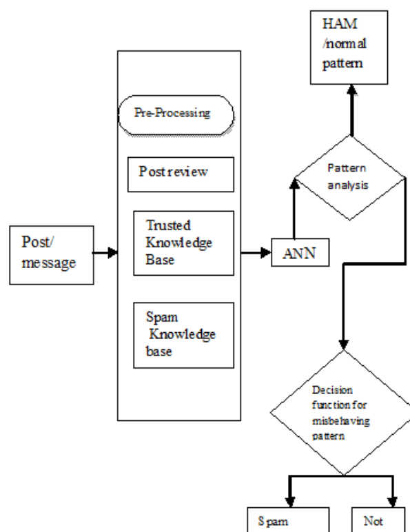
Fig. 1 Proposed Model
