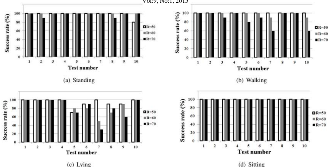
Fig. 4 Variation in correct classification success of the activities depending on random packet loss
