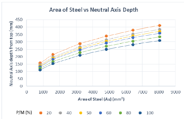
Fig. 5 Area of Steel vs Neutral Axis Depth
