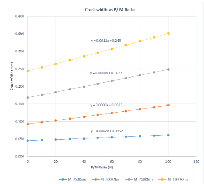
Fig. 2 Crack width vs P/M Ratio
