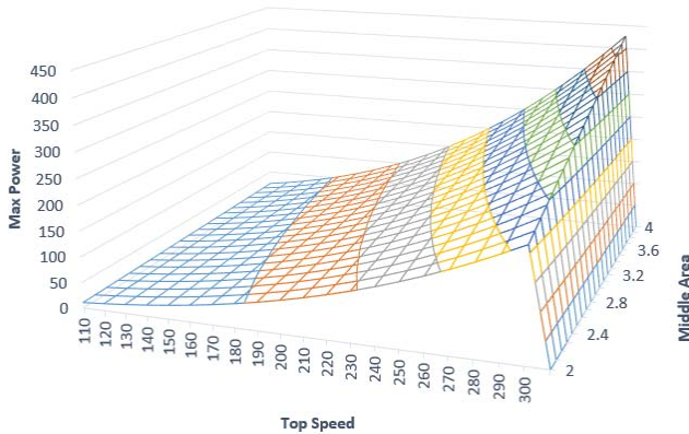
Fig. 2 Required Peak Motor Power
