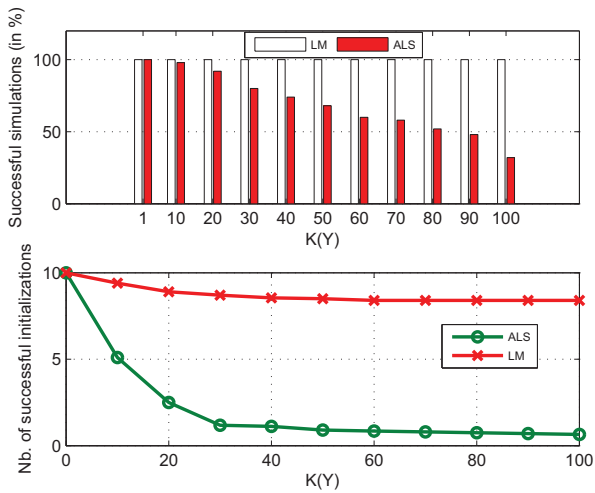
Fig. 3 Number of simulations and successful initializations
