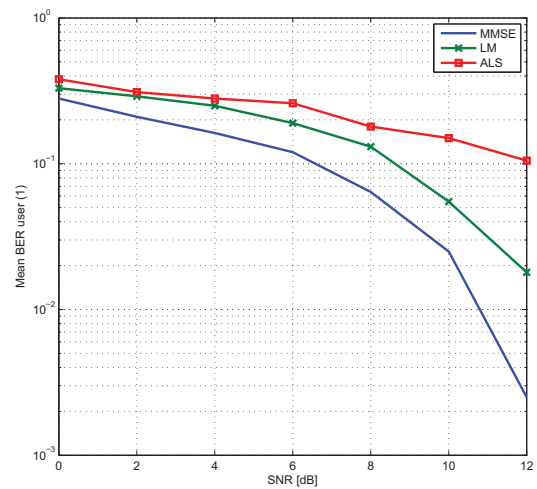
Fig. 4 BER of user 1
